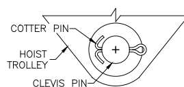
Diagram 2E. Installing cotter pin through retaining pin.
