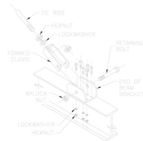
Diagram 2C. Bolting end of beam bracket to boom.
