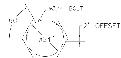
Diagram 3G. 6 bolt base bolt pattern.
