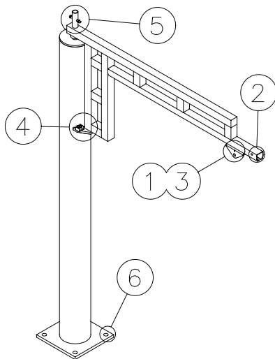
WSJ360 Free Standing Crane
