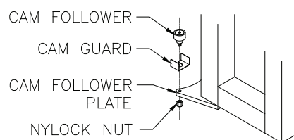
Diagram 4B. Installing cam followers.
