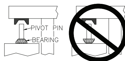
Diagram 4C. Orienting bearing.
