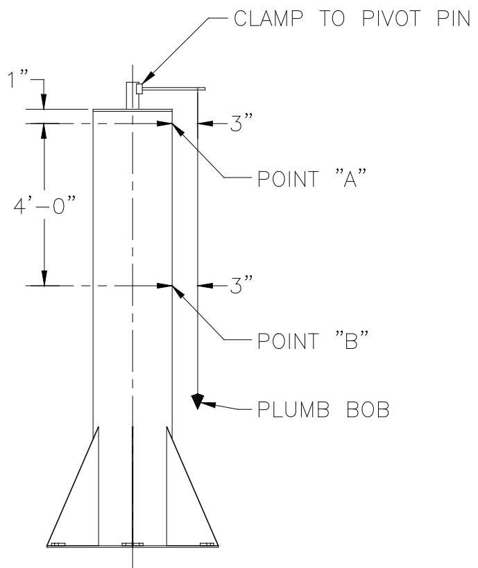
Diagram 3J. Plumbing the mast.
