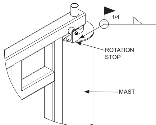
Diagram 9C. Welding rotation stops on the WSJ360.
