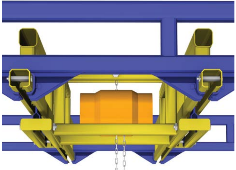
Nested Trolley
