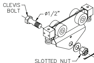
Diagram 6I. Installing hoist on A150 hoist trolley.
