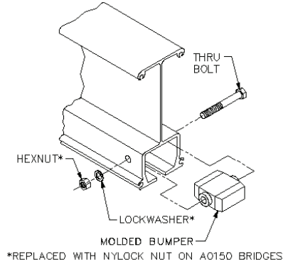
Diagram 7B. Re-installing endstop in track after installing festoon stack section.
