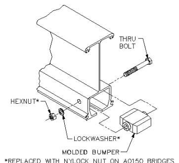
Diagram 8D. Installing endstop on runway/festoon stack section.
