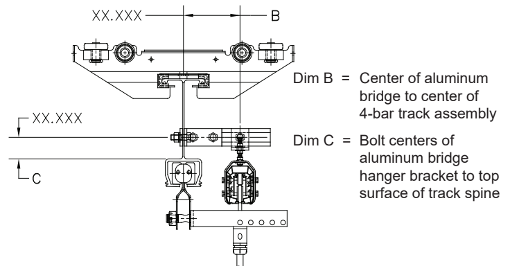
Diagram 10E. One piece aluminum bridge B-C dimensions.
