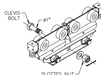
Diagram 6L. Installing hoist on A2000 loadbar hoist trolley.
