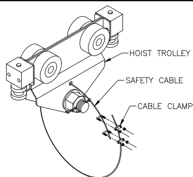
Diagram 6H. Installing safety cable on hoist trolley.
