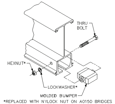
Diagram 5H. Installing end stop.
