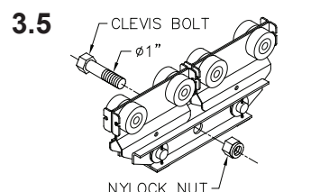
Diagram 3F. Installing hoist on A2000 hoist trolley.
