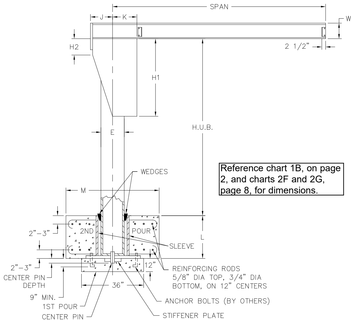
Diagram 2E. FS350S
