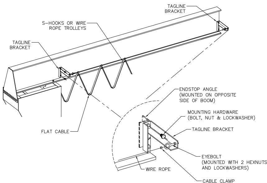
Diagram 6B. Tagline festoon installation.
