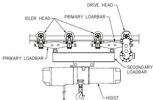
Diagram 6C. WT Carrier (4 Head).
