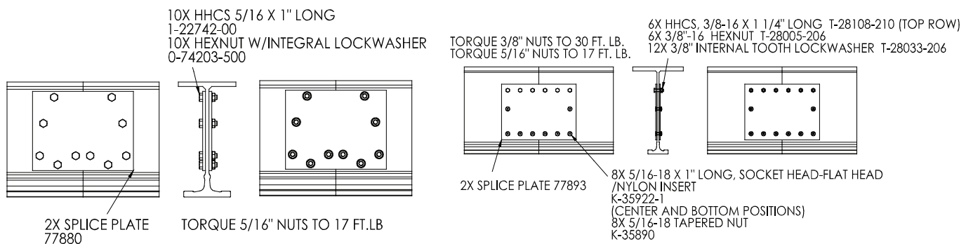
Diagram 3F. Bolted splice (4200 - 4600 Tarca® beam).
