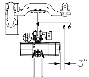
Diagram 7B. End view.
