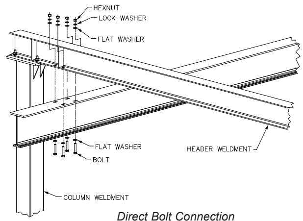
Diagram 4A. Attaching runway to header weldment.
