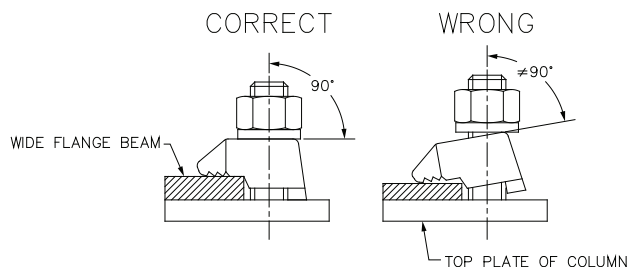
Diagram 3C. Beam Clamp Installation.
