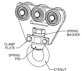
Diagram 6A. Tether Track® trolley installation.
