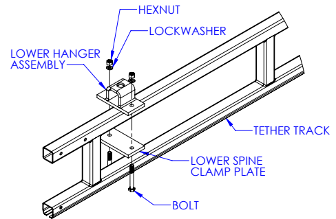
Diagram 5C. Attaching lower hanger assembly to monorail.
