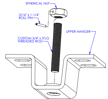
Diagram 5A. Assembling threaded rod to upper hanger.
