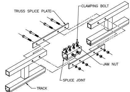
Diagram 5H. Splicing trussed track.
