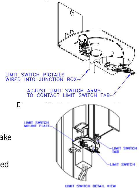
Diagram 9C. Limit switch detail.
