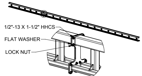
Diagram 5K. Plate style splice joint design.
