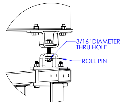
Diagram 5E. Leveling monorail.
