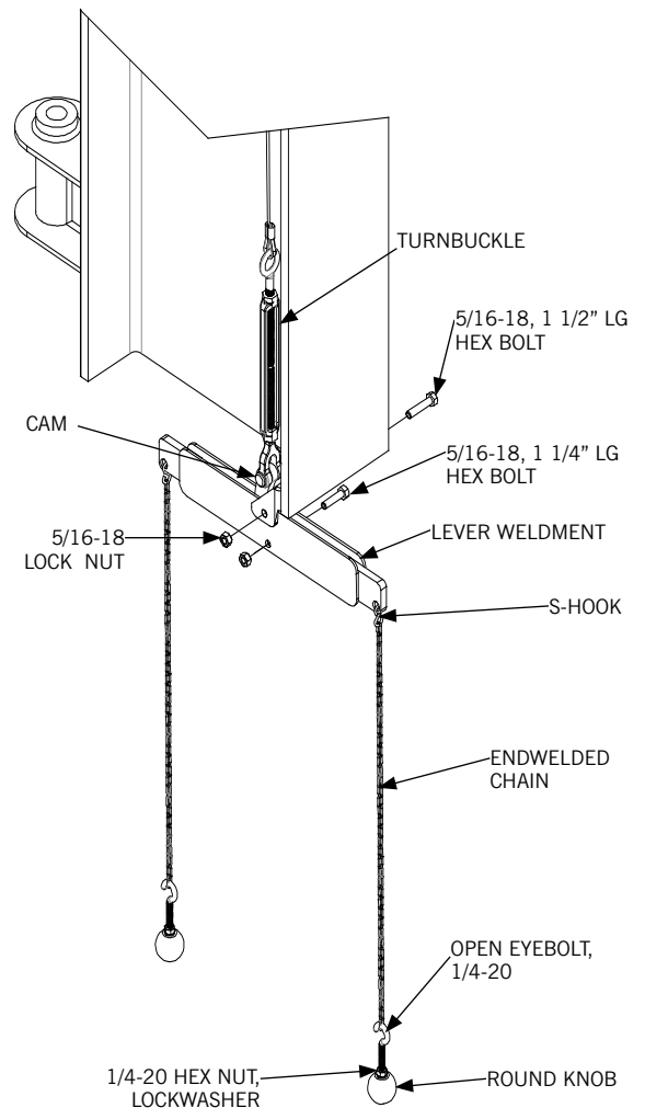
Diagram 7J. Lever installation.
