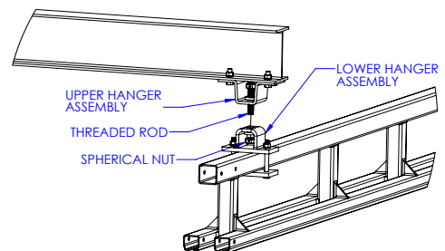
Diagram 5D. Attaching monorail to cantilever.
