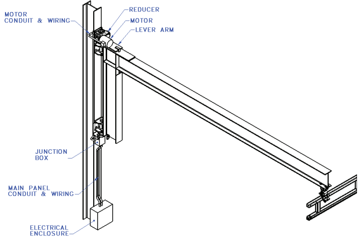
Diagram 8A. Drive installation.
