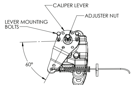
Diagram 7A. Brake caliper assembly.
