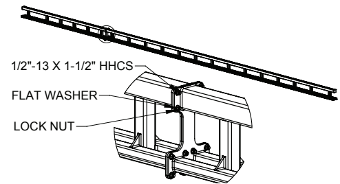
Diagram 5K. Plate style splice joint design.
