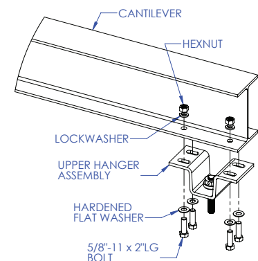
Diagram 5B. Attaching upper hanger to cantilever.
