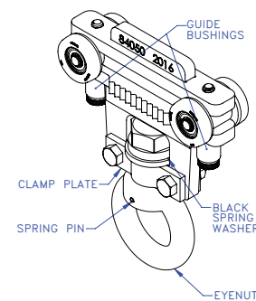
Diagram 6B. Recover trolley installation.
