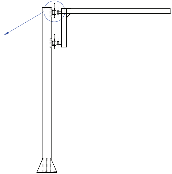
Diagram 4A. Attaching cantilever to mast.
