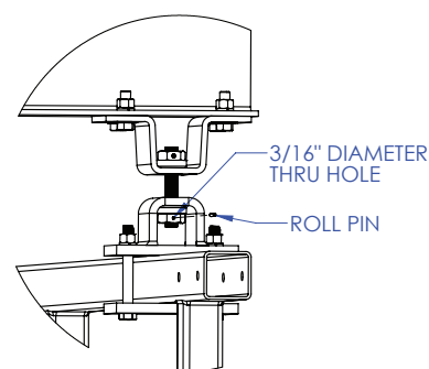
Diagram 5E. Leveling monorail.
