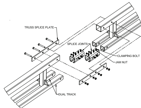
Diagram 5J. Splicing dual trussed track.
