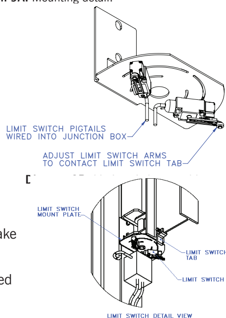
Diagram 9C. Limit switch detail.
