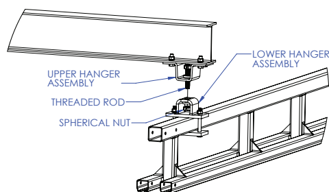
Diagram 5D. Attaching monorail to cantilever.
