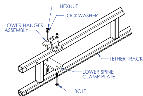
Diagram 5C. Attaching lower hanger assembly to monorail.
