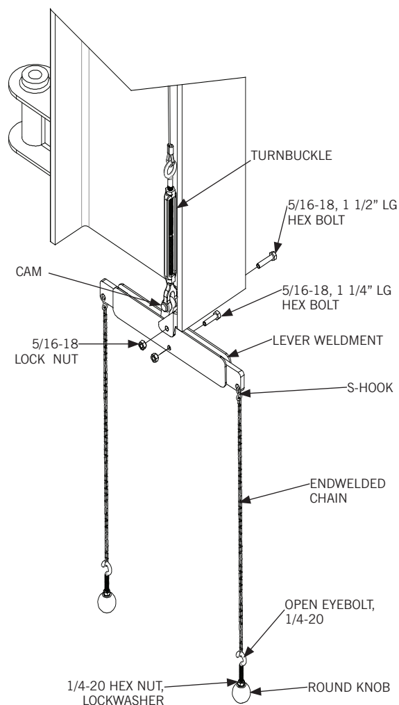
Diagram 7J. Lever installation.
