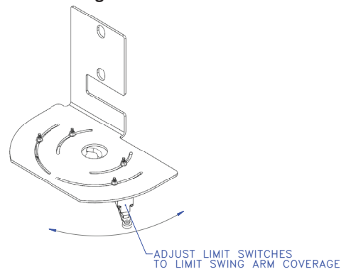
Diagram 9D. Limit switch adjustment.
