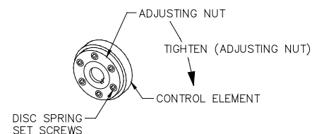
Diagram 8C. Indoor clutch torque adjustment.
