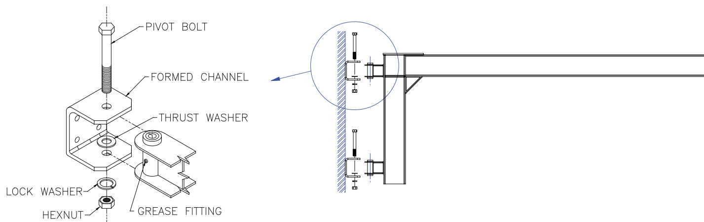
Diagram 2B. Attaching cantilever assembly to formed channel.
