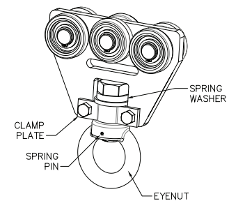
Diagram 6A. Tether Track® trolley installation.
