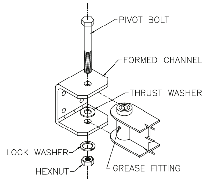
Diagram 4A. Attaching cantilever to mast.
