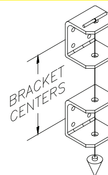
Diagram 2A. Plumbing formed channel brackets.
