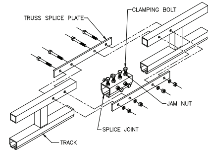
Diagram 5H. Splicing trussed track.
