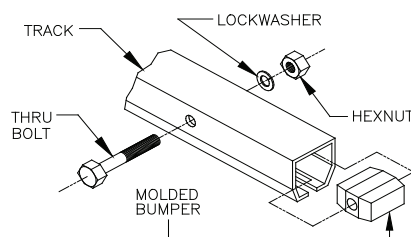
Diagram 5G. Installing end stop.
