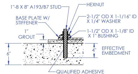
Diagram 3D. Anchor bolt installation.
