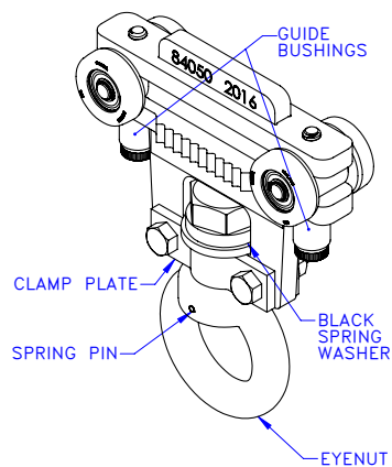
Diagram 6A. Tether Track® trolley installation.
