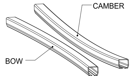
Diagram B. Camber and Bow.
