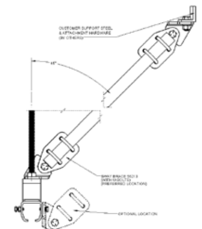
Diagram 3. Typical Connection detail.
