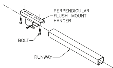
Perpendicular Flush Mount
