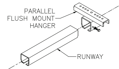
Parallel Flush Mount
