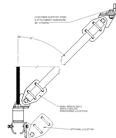
Diagram 3. Typical Connection detail.
