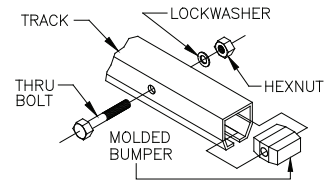
Diagram 5D. Installing end stop.
