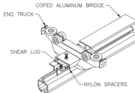
Diagram 5B. Installing clamping end truck on coped aluminum bridge. See TIP .
