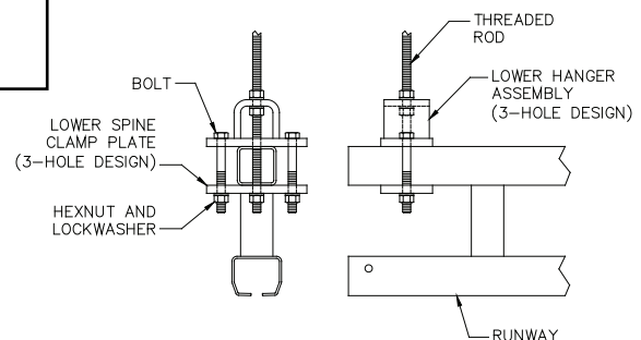
Diagram 3E. 3-Hole Hanger.
