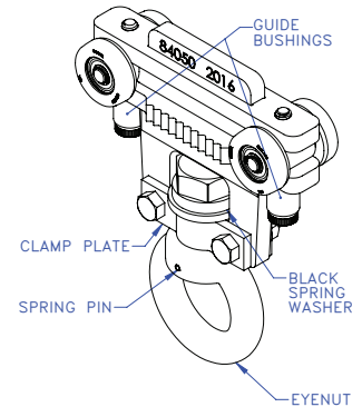
Diagram 6A. Tether Track® trolley installation.
