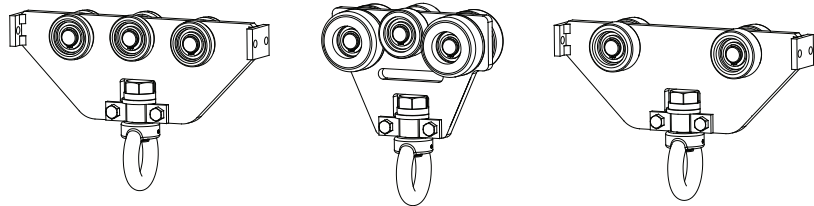
Diagram 6B. Various monorail and bridge trolley configurations.
