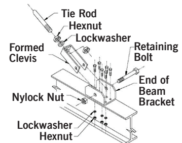
Diagram 2C. Bolting end of beam bracket to boom.
