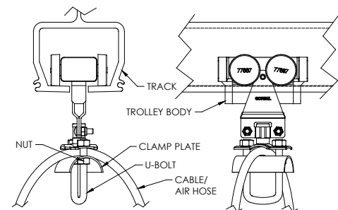
Diagram 6B. Installing electric cable/air hose on festoon trolley.
