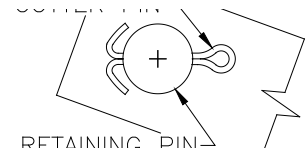
Diagram 5E. Installing cotter pin through trolley saddle clevis pin.
