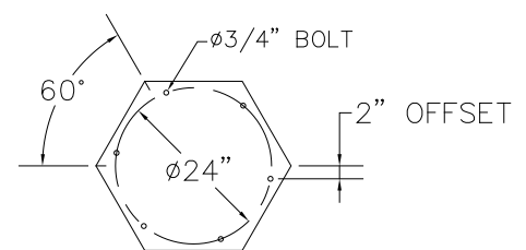
Diagram 3G. 6 bolt base bolt pattern.
