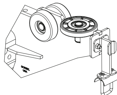
Diagram 5D. Installing tow arm on end truck.
