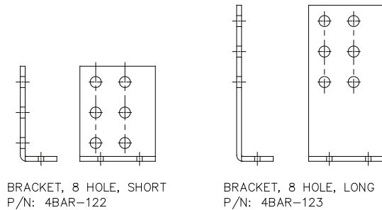
Diagram 10C. Bridge brackets.
