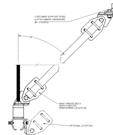
Diagram 1. Typical Connection detail.
