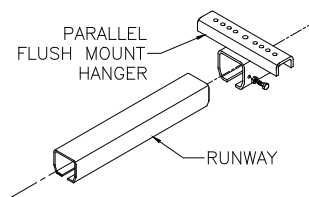
Parallel Flush Mount 250-2000#
