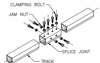
Diagram 4A. Splicing untrussed track.
