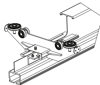
Diagram 5C. Installing clamping end truck on coped aluminum bridge.
